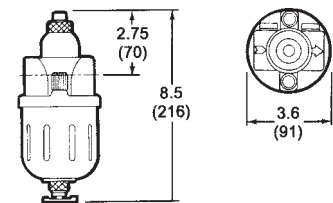
Manual Drain
